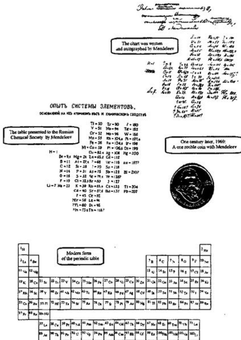
Figure 2 The Periodic Table of the elements.
