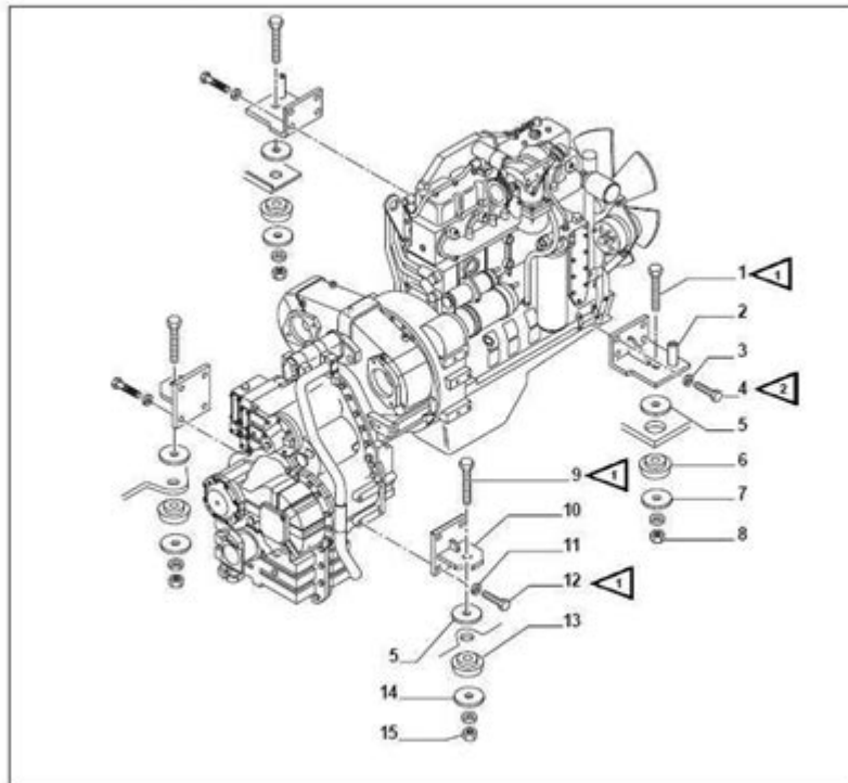
Fig. 1-6 Engine supports
