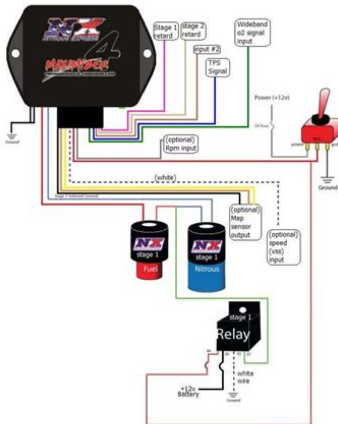
Single Stage Wiring WITH Wide-Band o2 AFR Correction:
