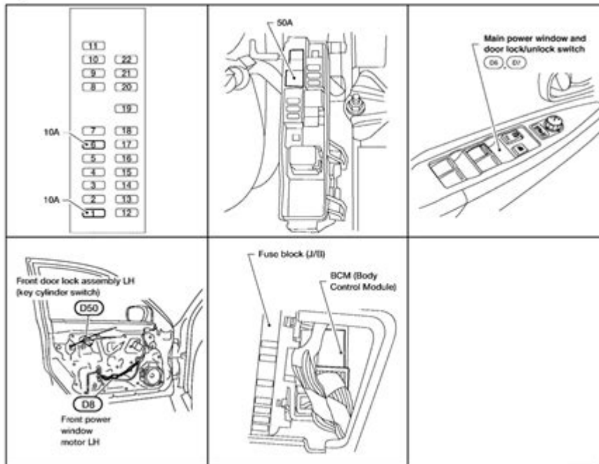
Component Parts and Harness Connector Location
