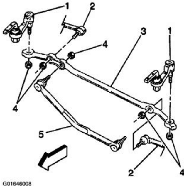
Fig. 41: Installing Prevailing Torque Nut To Idler Arm Ball Studs Courtesy of GENERAL MOTORS CORP.
