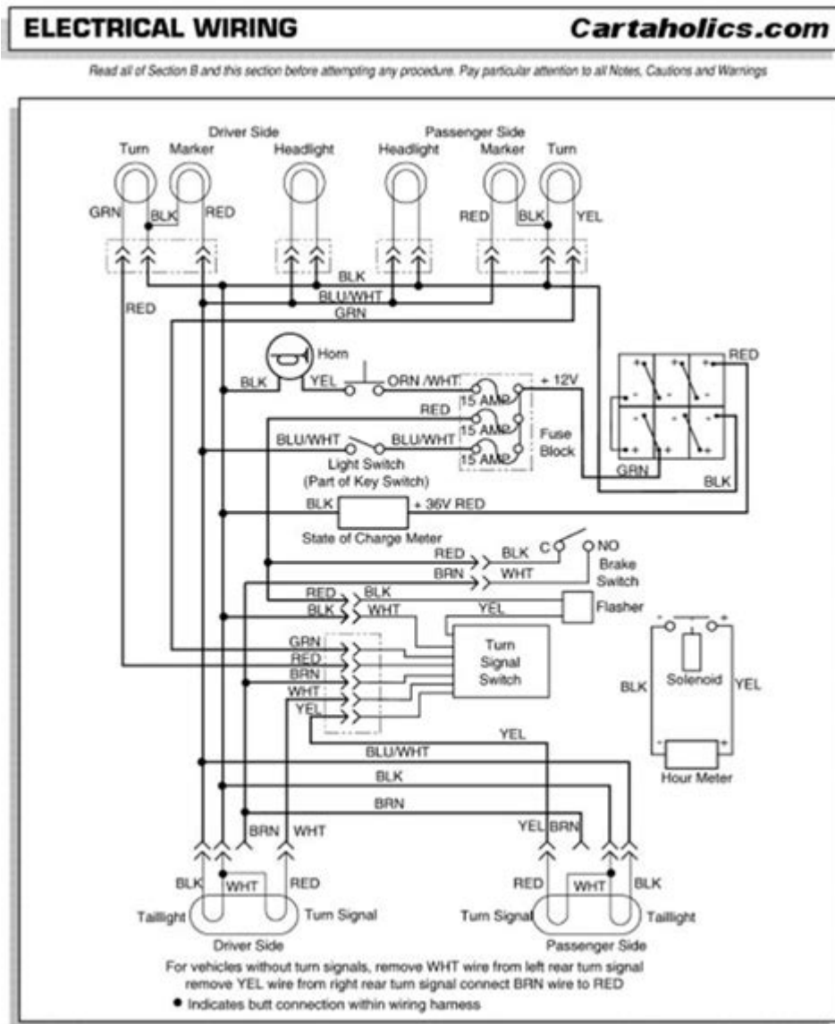
Fig. 2 Accessory Wiring Diagram
