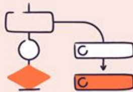
Decision trees
