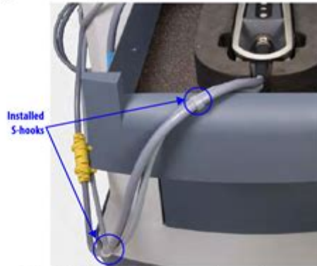
Figure 4.9 S-hooks to hold camera cables together
