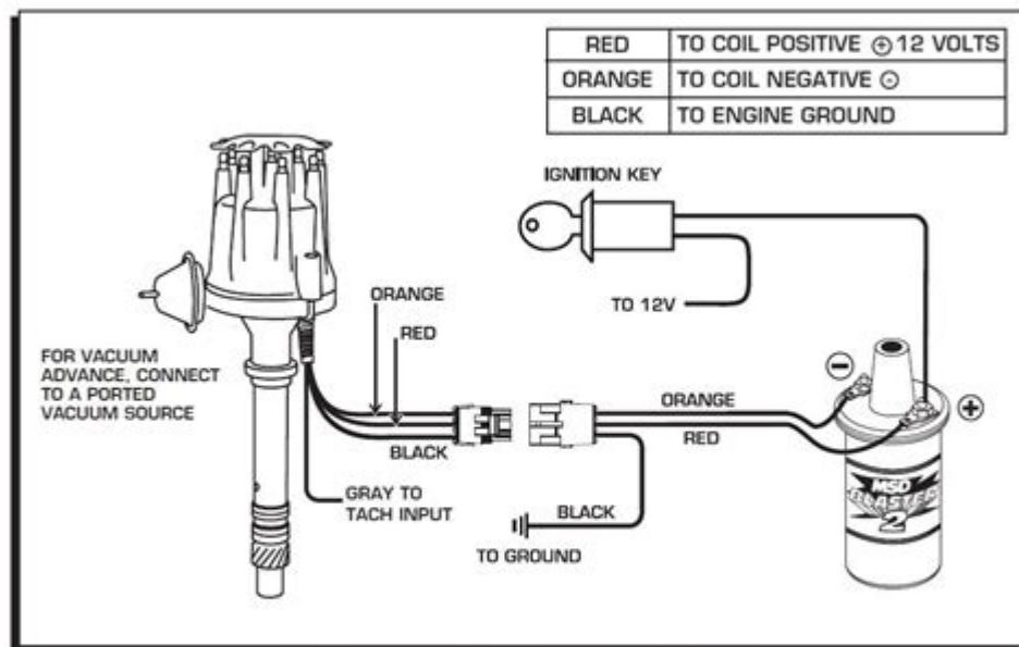
Figure 10 Wiring the Ready-to-Run Chevrolet Distributor.
