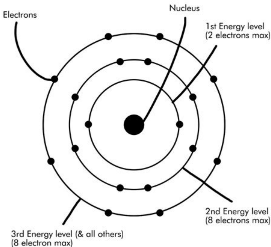
Electron Energy Levels
