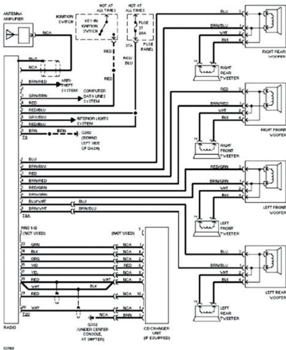
2001 Volkswagen Passat Radio w/o Monsoon Radio Circuit
