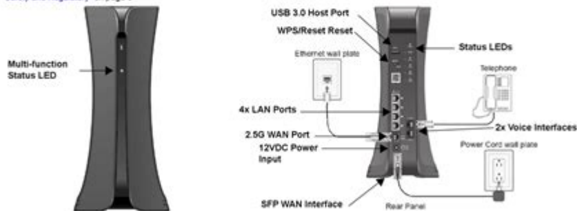
Figure 1. 854-(v)6 Router
