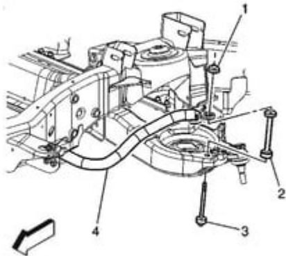
Fig. 5: Removing The Stabilizer Shaft Link Courtesy of GENERAL MOTORS CORP.
