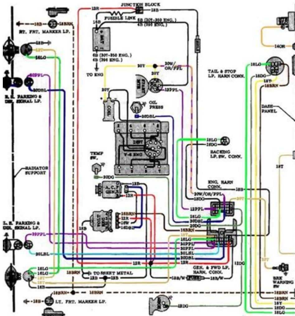
1970 Chevelle Wiring Diagram
