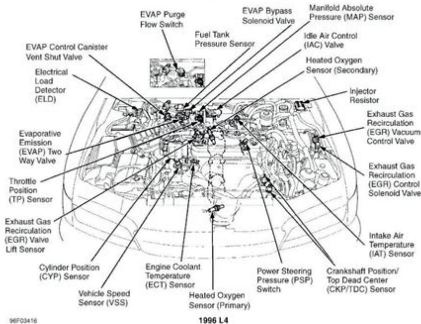
1996 Honda Accord EX Fig. 5: Engine Compartment (1996) (2.2L)
