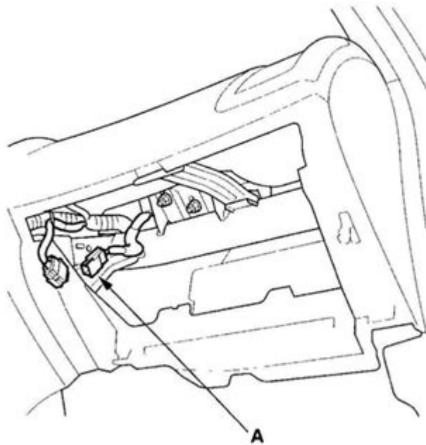
Fig. 28: Disconnecting Front Passenger's Airbag 4P Connector From Dashboard Wire Harness (Front Passenger's Airbag) Courtesy of AMERICAN HONDA MOTOR CO., INC.
