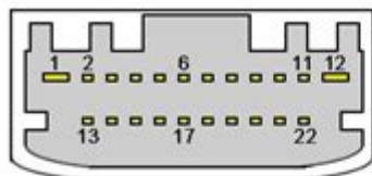
22 pin Dodge, Jeep Head Units connector
