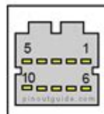
10 pin Jeep Head Unit Audio connector
